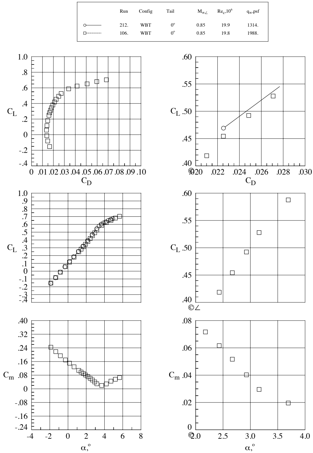
Figure 14. Aeroelastic effects, WBT0 Configuration, Mach = 0.85, Re_c = 19.8 \times 10^6 .
