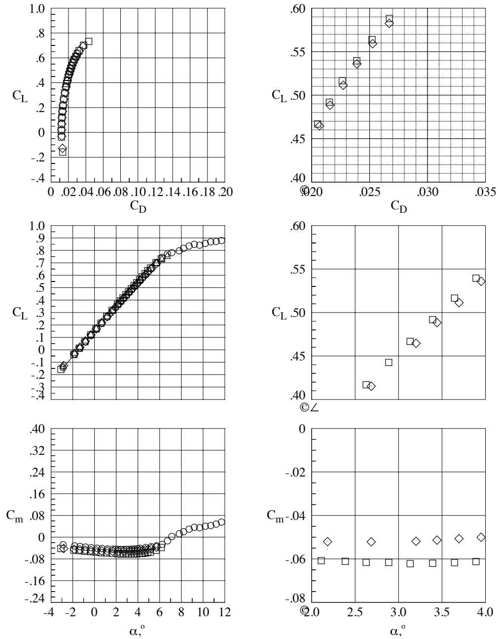
Figure 20. Reynolds Number Effects, WB Configuration, Mach = 0.7.
