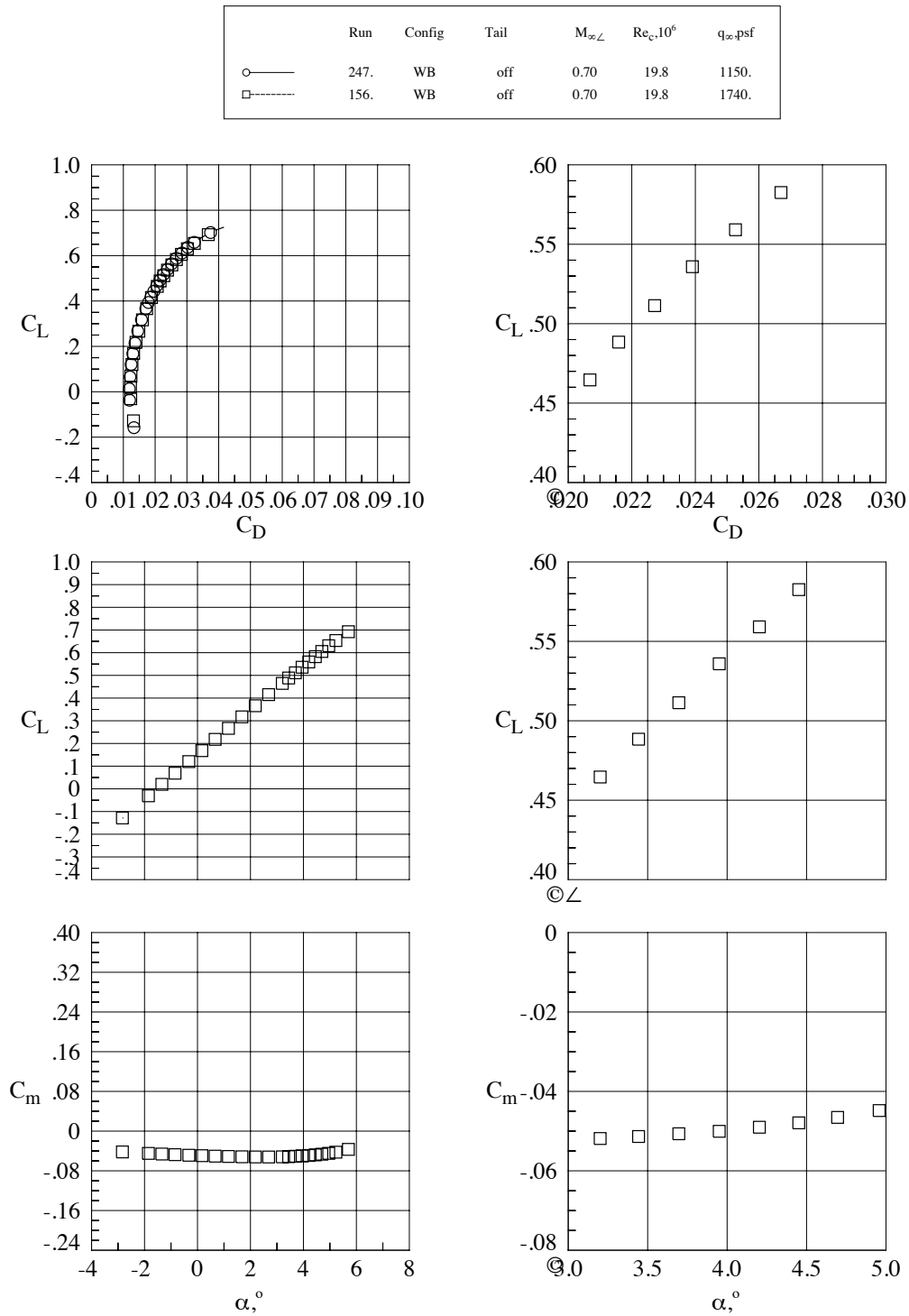
Figure 11. Aeroelastic effects, WB Configuration, Mach = 0.7, Re_c = 19.8 \times 10^6 .
