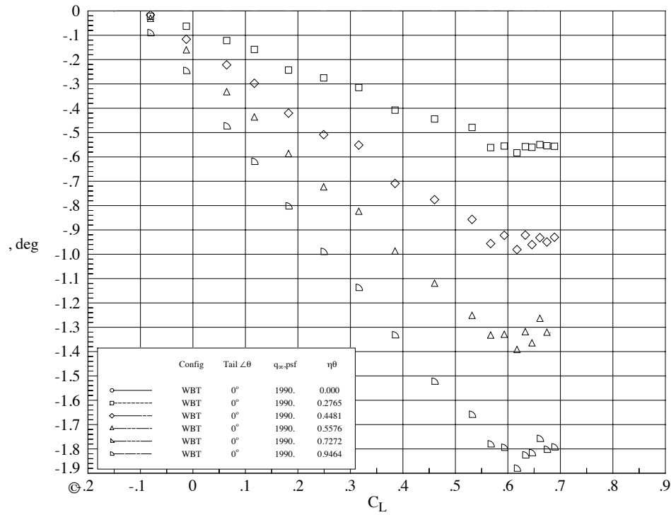
Figure 8. Model Deformation, WBT0 Configuration, Mach = 0.85, Re_c = 30 \times 10^6 , high q_\infty .
