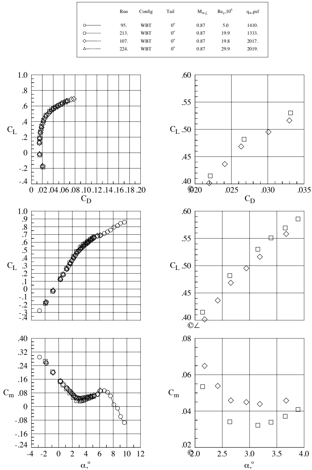
Figure 25. Reynolds Number Effects, WBT0 Configuration, Mach = 0.87.
