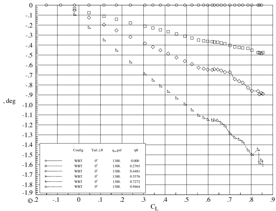
Figure 5. Model Deformation, WBT0 Configuration, Mach = 0.85, Re_c = 5 \times 10^6 , low q_\infty .
