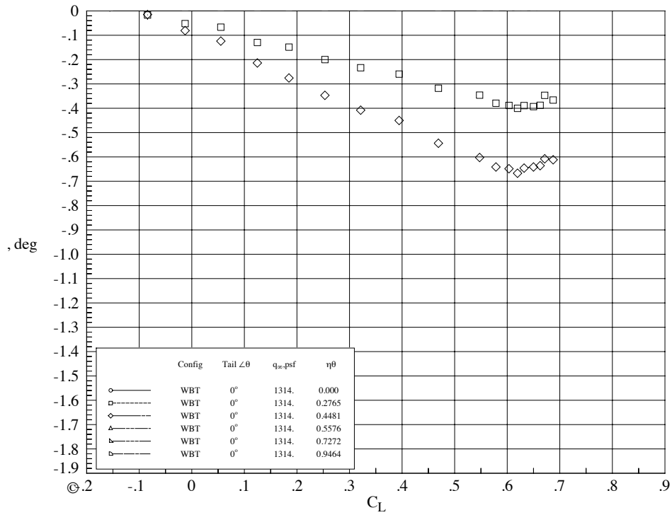
Figure 6. Model Deformation, WBT0 Configuration, Mach = 0.85, Re_c = 19.8 \times 10^6 , low q_\infty .
