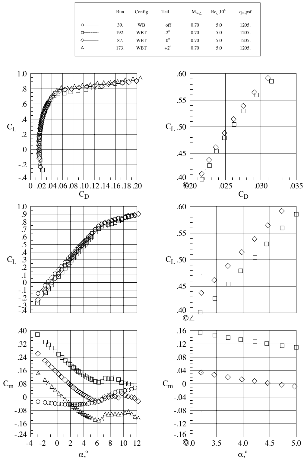
Figure 26. Tail Effects, Mach = 0.7, Re_c = 5 \times 10^6 .
