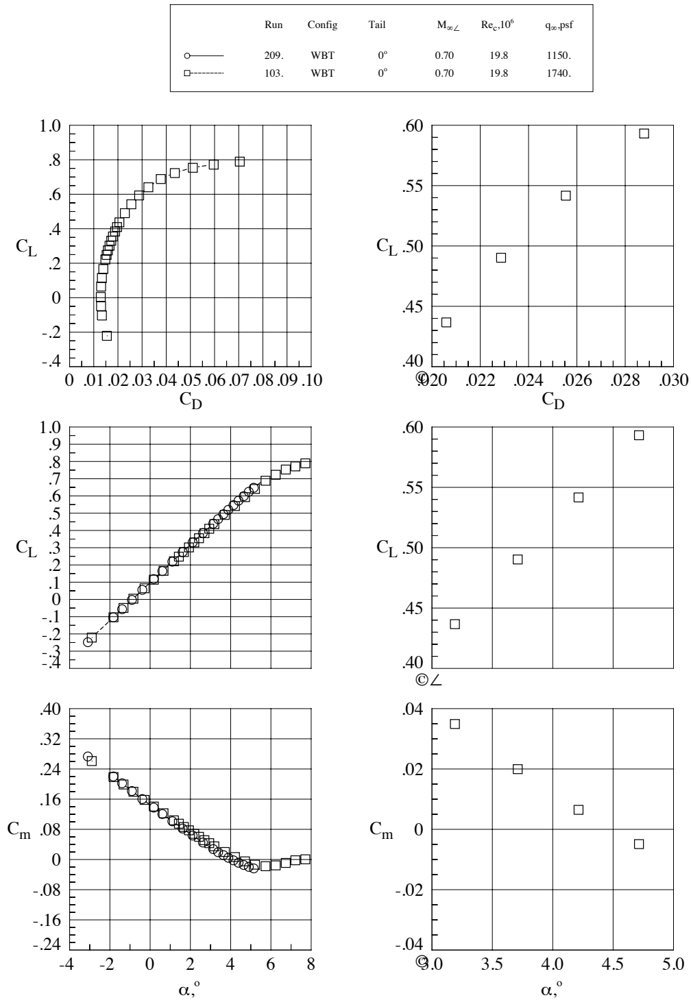
Figure 12. Aeroelastic effects, WBT0 Configuration, Mach = 0.7, Re_c = 19.8 \times 10^6 .
