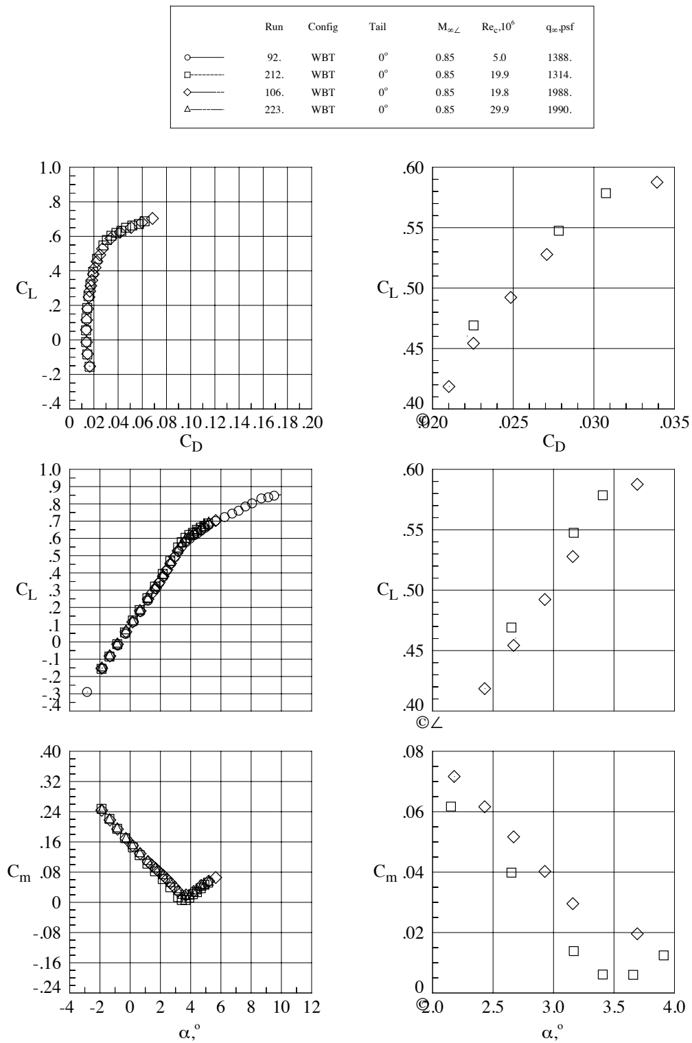
Figure 23. Reynolds Number Effects, WBT0 Configuration, Mach = 0.85.
