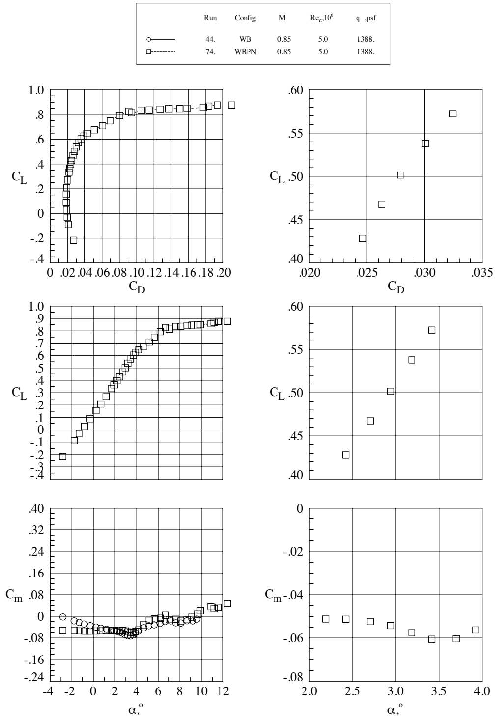
Figure 18. Nacelle/Pylon Effects, Mach = 0.85, Re_c = 5 \times 10^6 .
