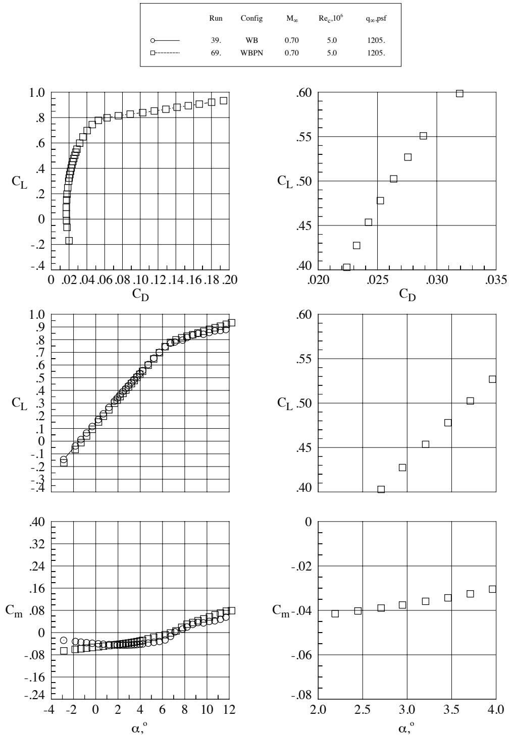
Figure 17. Nacelle/Pylon effects, Mach = 0.7, Re_c = 5 \times 10^6 .
