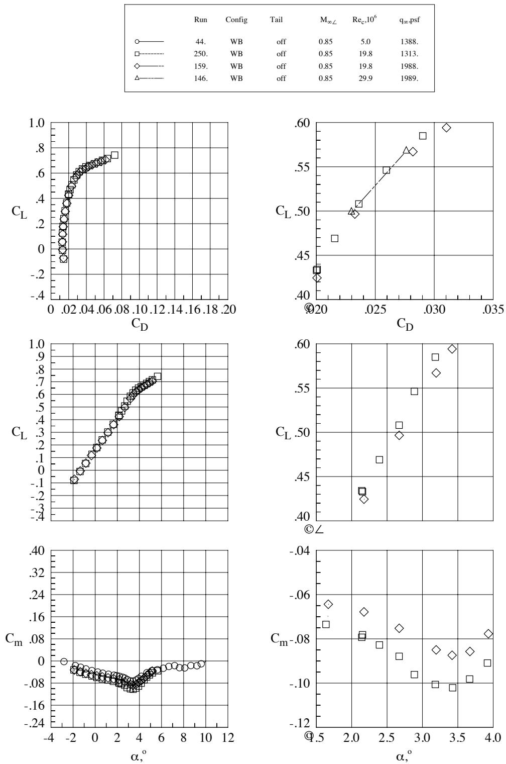
Figure 22. Reynolds Number Effects, WB Configuration, Mach = 0.85.
