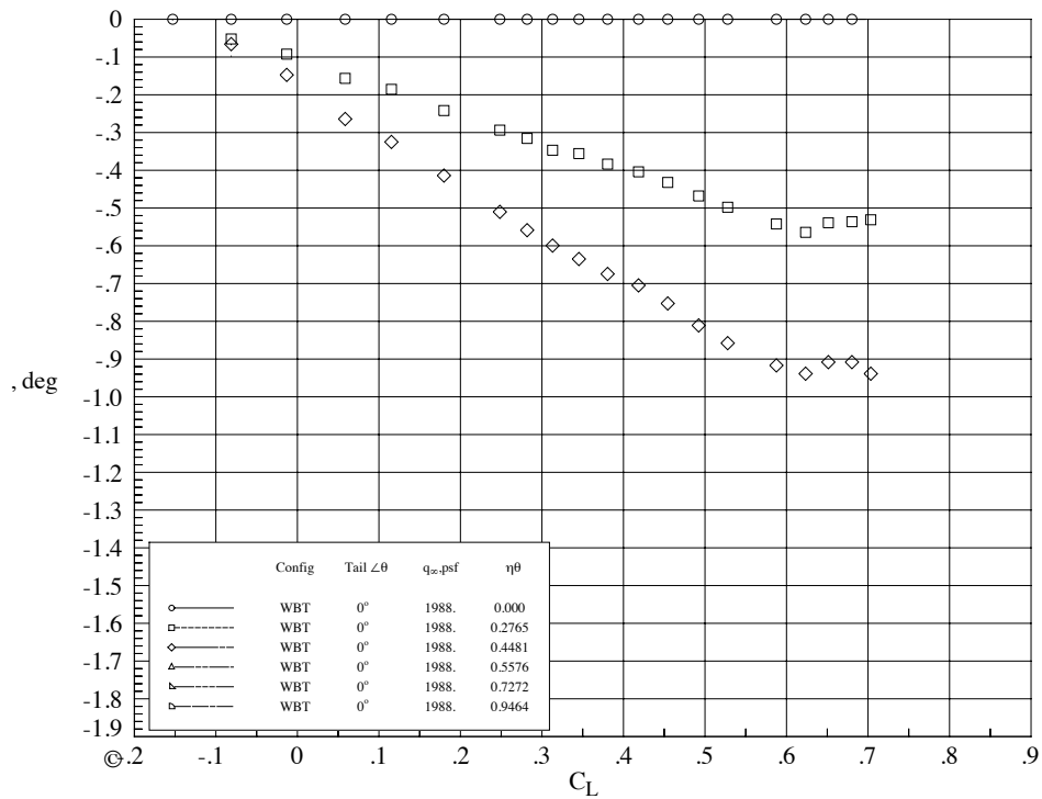
Figure 7. Model Deformation, WBT0 Configuration, Mach = 0.85, Re_c = 19.8 \times 10^6 , high q_\infty .
