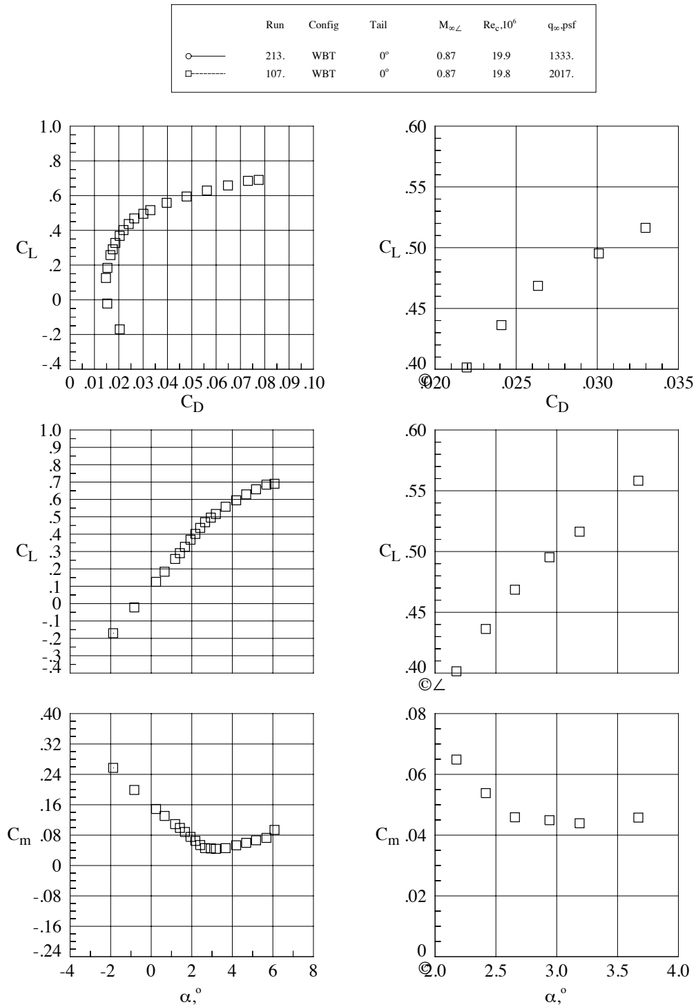
Figure 16. Aeroelastic effects, WBT0 Configuration, Mach = 0.87, Re_c = 19.8 \times 10^6 .
