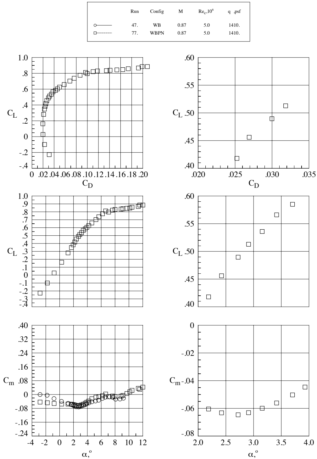
Figure 19. Nacelle/Pylon Effects, Mach = 0.87, Re_c = 5 \times 10^6 .
