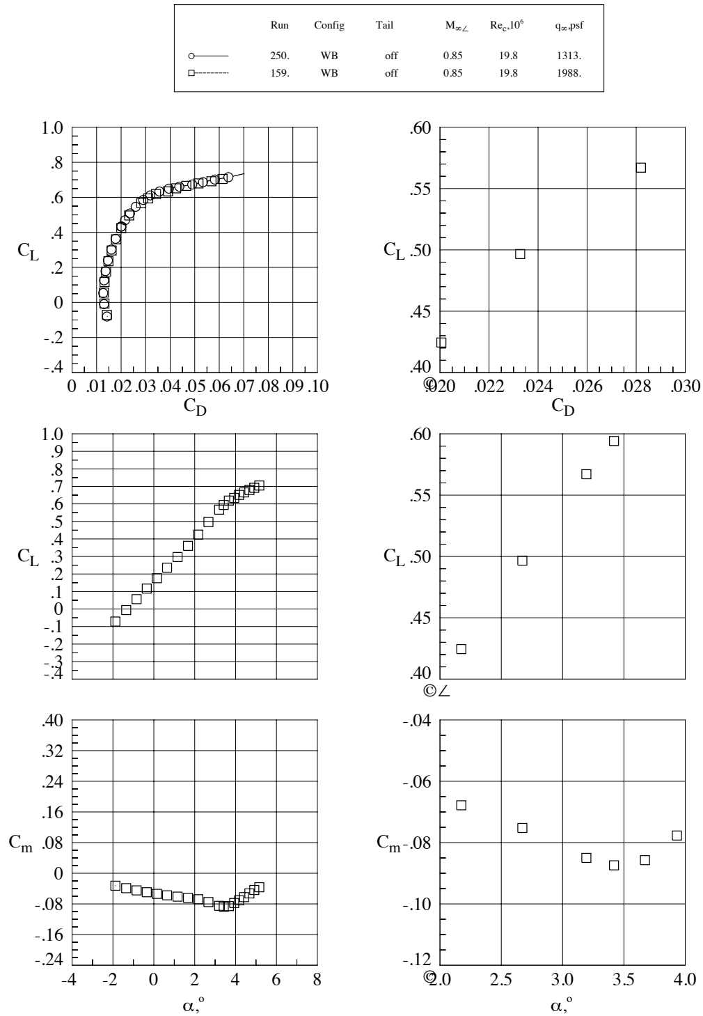
Figure 13. Aeroelastic effects, WB Configuration, Mach = 0.85, Re_c = 19.8 \times 10^6 .
