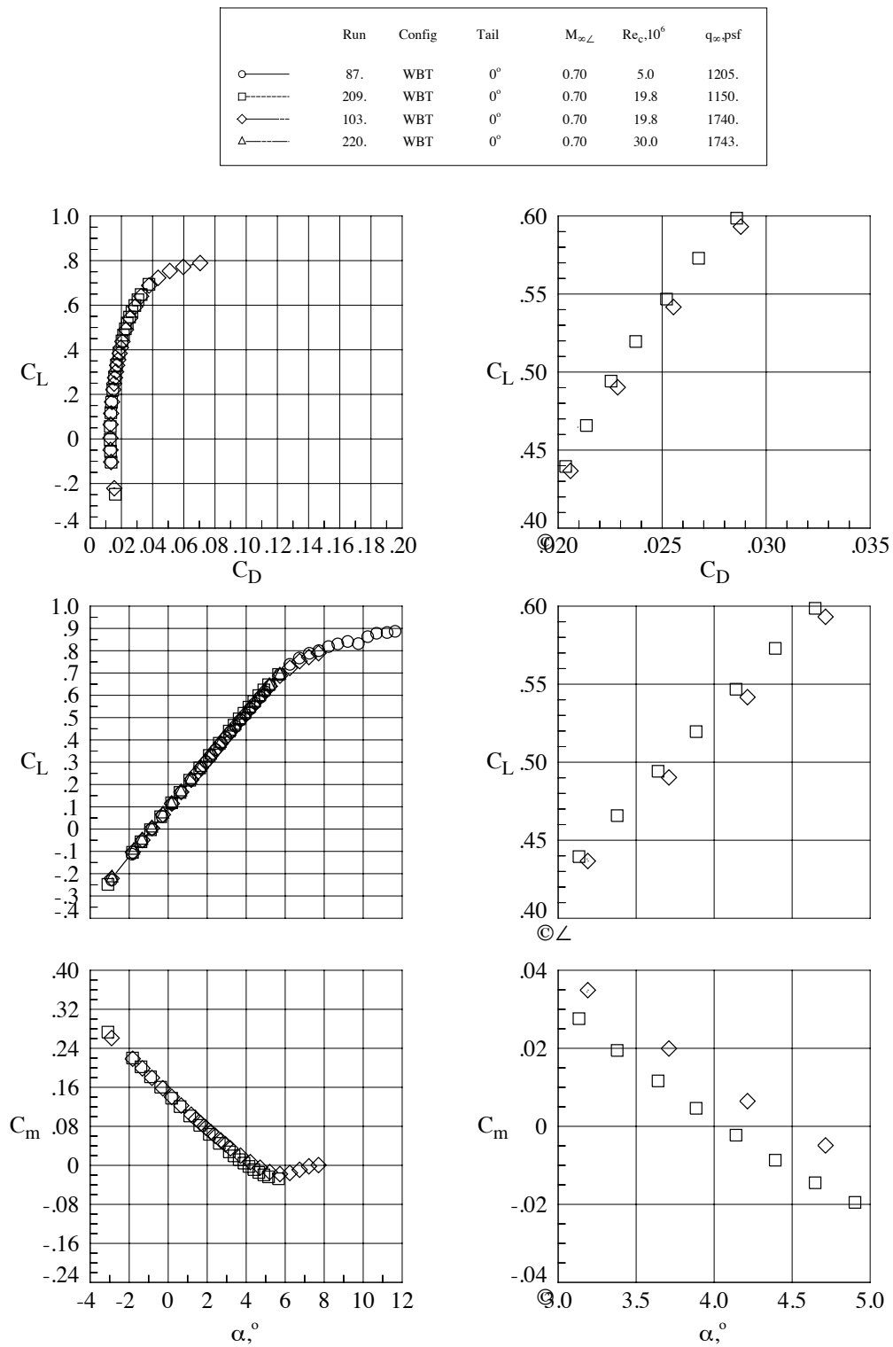
Figure 21. Reynolds Number Effects, WBT0 Configuration, Mach = 0.7.
